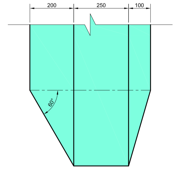
PIANO INTERIOR - PLANTA E 1:10
